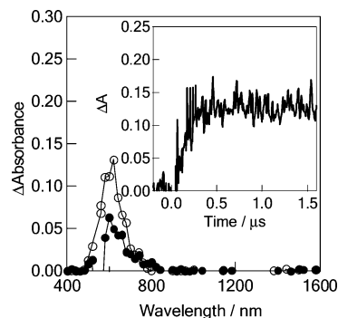
Figure 6. Nanosecond transient absorption spectra of SWNT/Pyr- NH_3^+ /crown- C_{60} (0.1 mM) in the presence of 0.5 mM HV^{2+} and 1.5 mM BNAH observed by 532 nm (ca. 3 mJ/pulse) laser irradiation in DMF (at 0.1 \mu s (●) and 1.0 \mu s (○)). (Inset) Absorption-time profile of the 620 nm peak.
